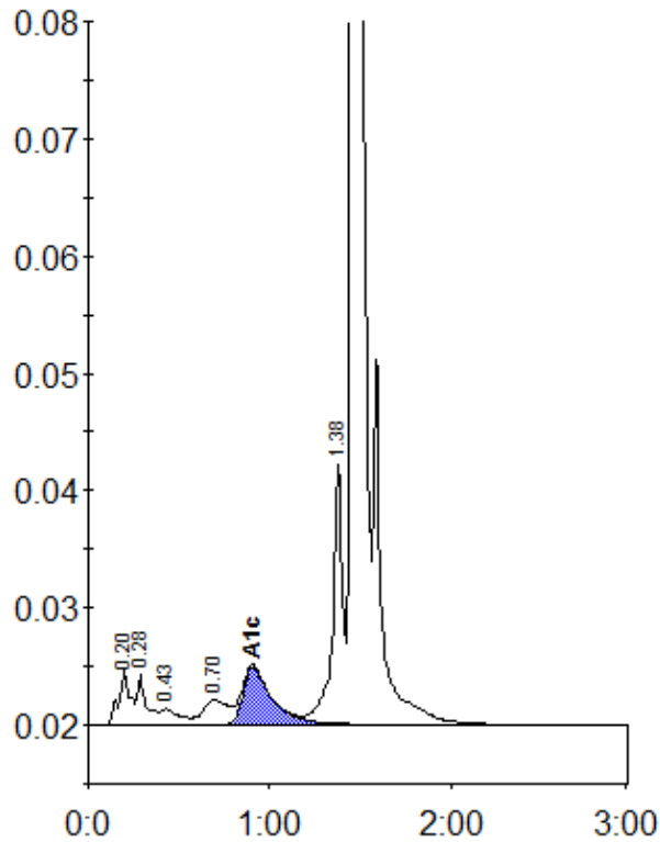
Peak table - ID: 10352409
